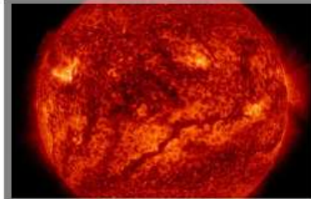
A dark, snaking line across the lower half of the sun in this image, captured by NASA's Solar Dynamics Observatory on Feb. 10, 2015, shows a filament of solar material hovering above the sun's surface. CREDIT: NASA/SDO
