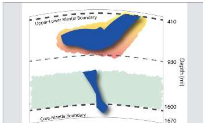
A simplified image of a slab from one of Earth's tectonic plates sinking through the upper mantle above, through the boundary between the upper ... [show more]
