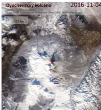
Satellite image of Klyuchevskoy volcano on 4 Nov 2016
