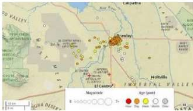
This map, generated about 5 p.m. on Jan. 1, 2017, shows the Brawley earthquake swarm that began on New Year's Eve. (U.S. Geological Survey)
