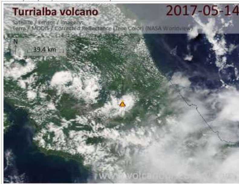
Satellite image of Turrialba volcano on 14 May 2017
