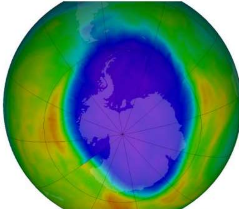
Above: The Antarctic ozone hole in Sept. 2016. [more]
