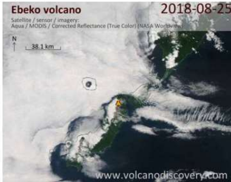
Satellite image of Ebeko volcano on 25 Aug 2018
