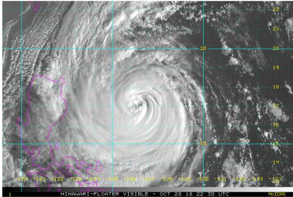
Typhoon Yutu on Oct. 28. Source: NOAA
