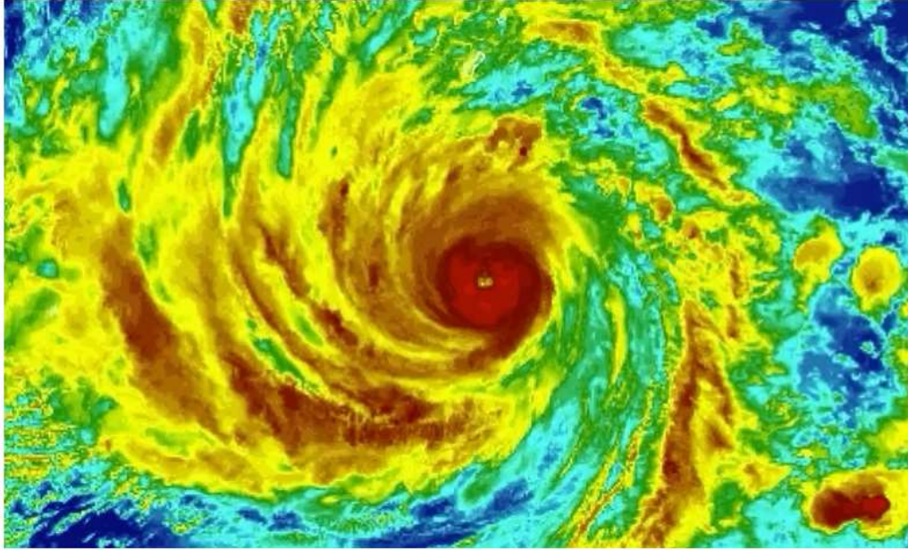
A satellite view of Typhoon Wutip with Guam visible to the north.
