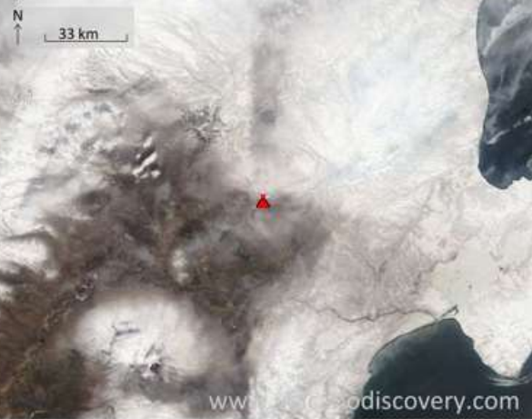
Satellite image of Shiveluch volcano on 13 May 2019
