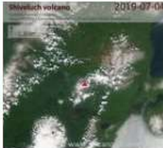
Satellite image of Shiveluch volcano on 4 Jul 2019
