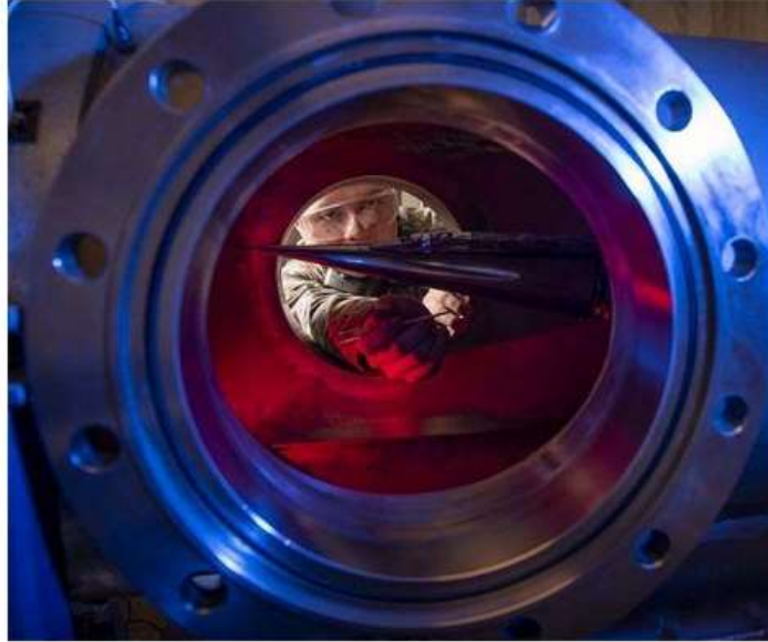
Cadet 2nd Class Eric Hembling uses a Ludwig Tube to measure the pressures, temperatures, and flow field of various basic geometric and hypersonic research vehicles at Mach 6 in The United States Air Force Academy's Department of Aeronautics, Thursday, Jan. 31, 2019
