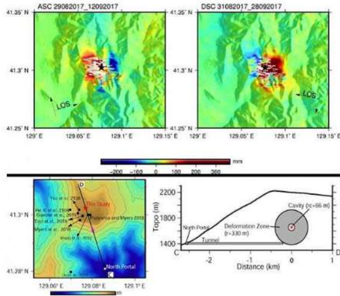
(Top) InSAR data in ascending and descending orbits depicting surface deformation associated with the 2017 nuclear test. (Bottom) Comparison of the source location of the 2017 nuclear test estimated from this study (red star) with other estimations. Topography along profile CD showing the cavity, deformation zone and probable location of tunnel. Note that the sizes of the cavity and deformation zones are exaggerated by 5 times for better visualisation.
