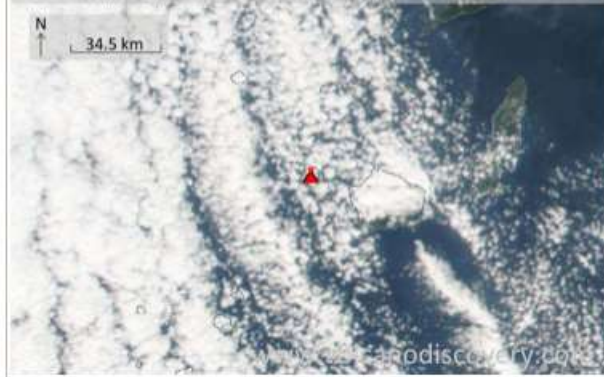
Satellite image of Kuchinoerabu-jima volcano on 9 Feb 2020
