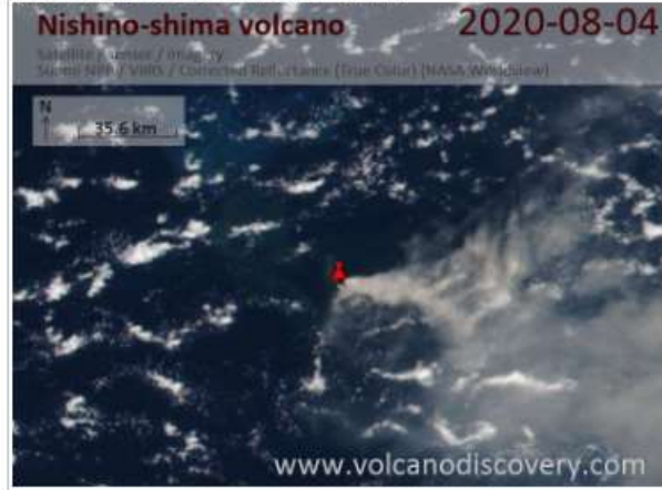
Satellite image of Nishino-shima volcano on 5 Aug 2020
