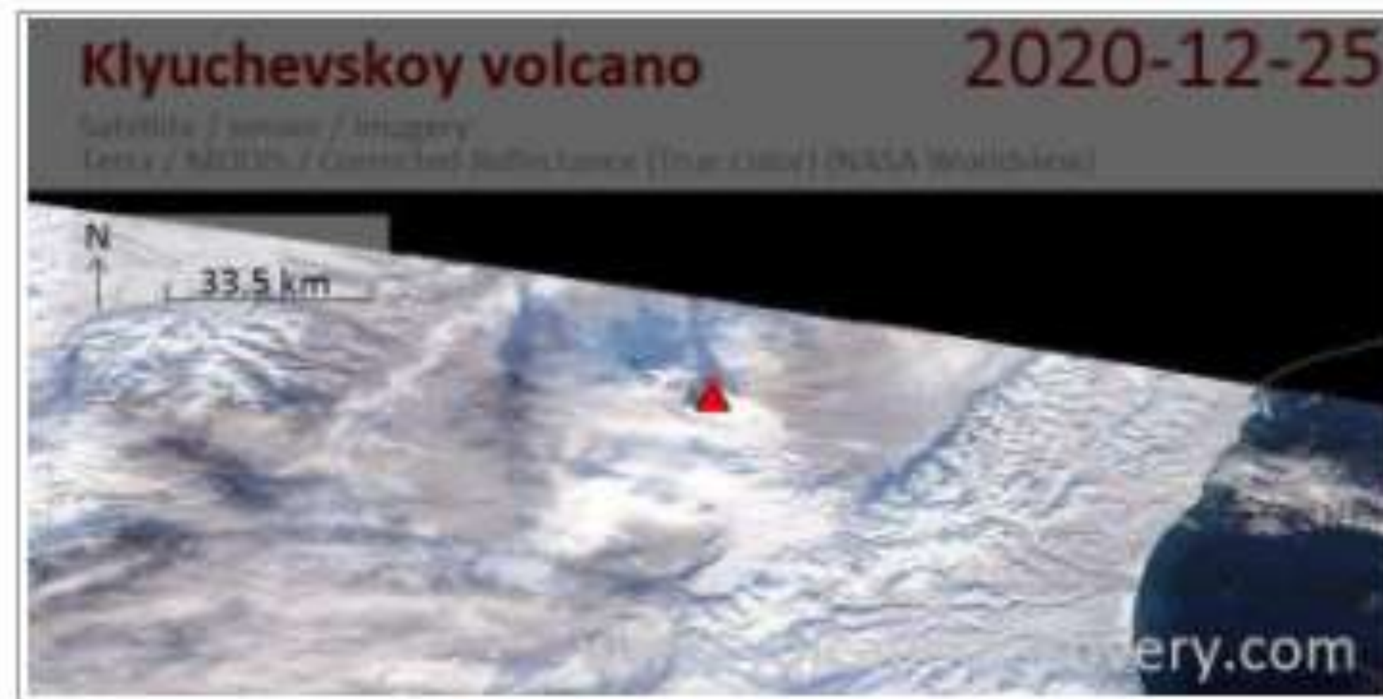
Satellite image of Klyuchevskoy volcano on 25 Dec 2020
