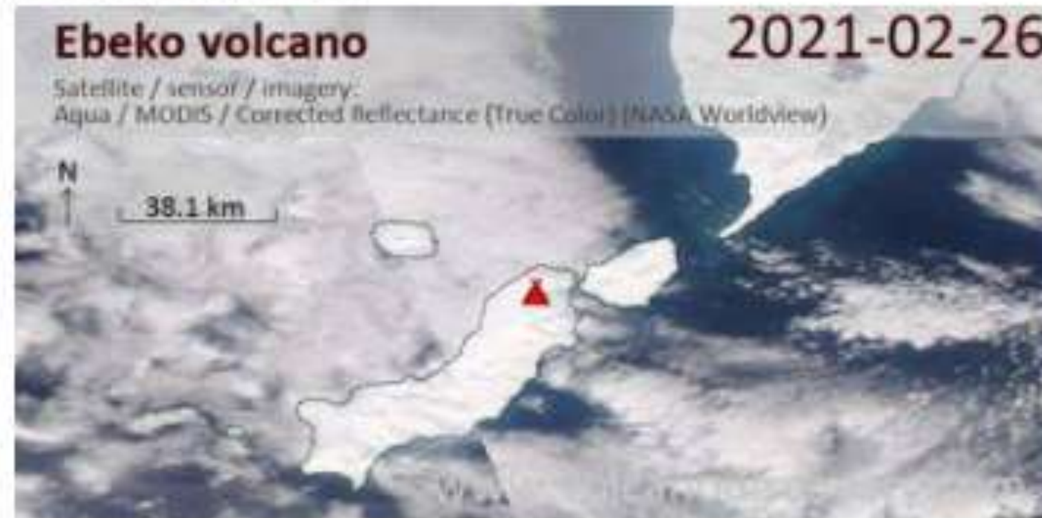
Satellite image of Ebeko volcano on 26 Feb 2021
