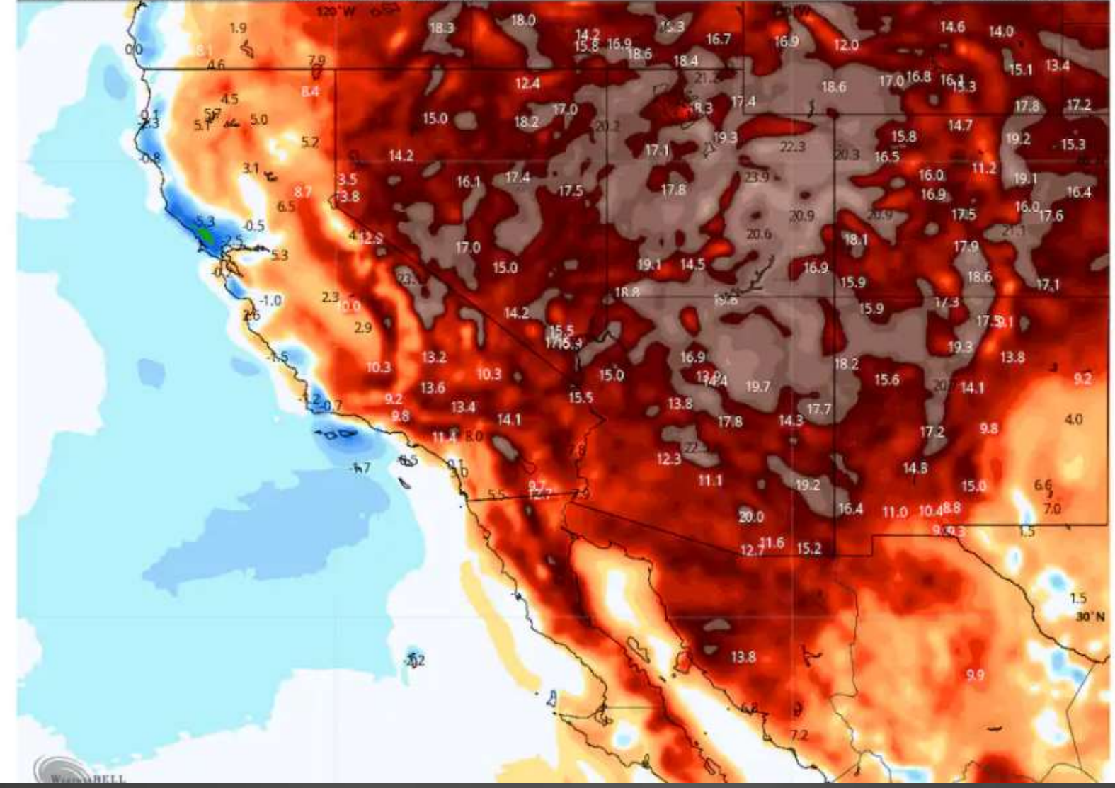
GFS 0.12° Init 06z 2 Apr 2021 • 2m Temperature Anomaly (°F) Hour: 54 • Valid: 12z Sun 4 Apr 2021
