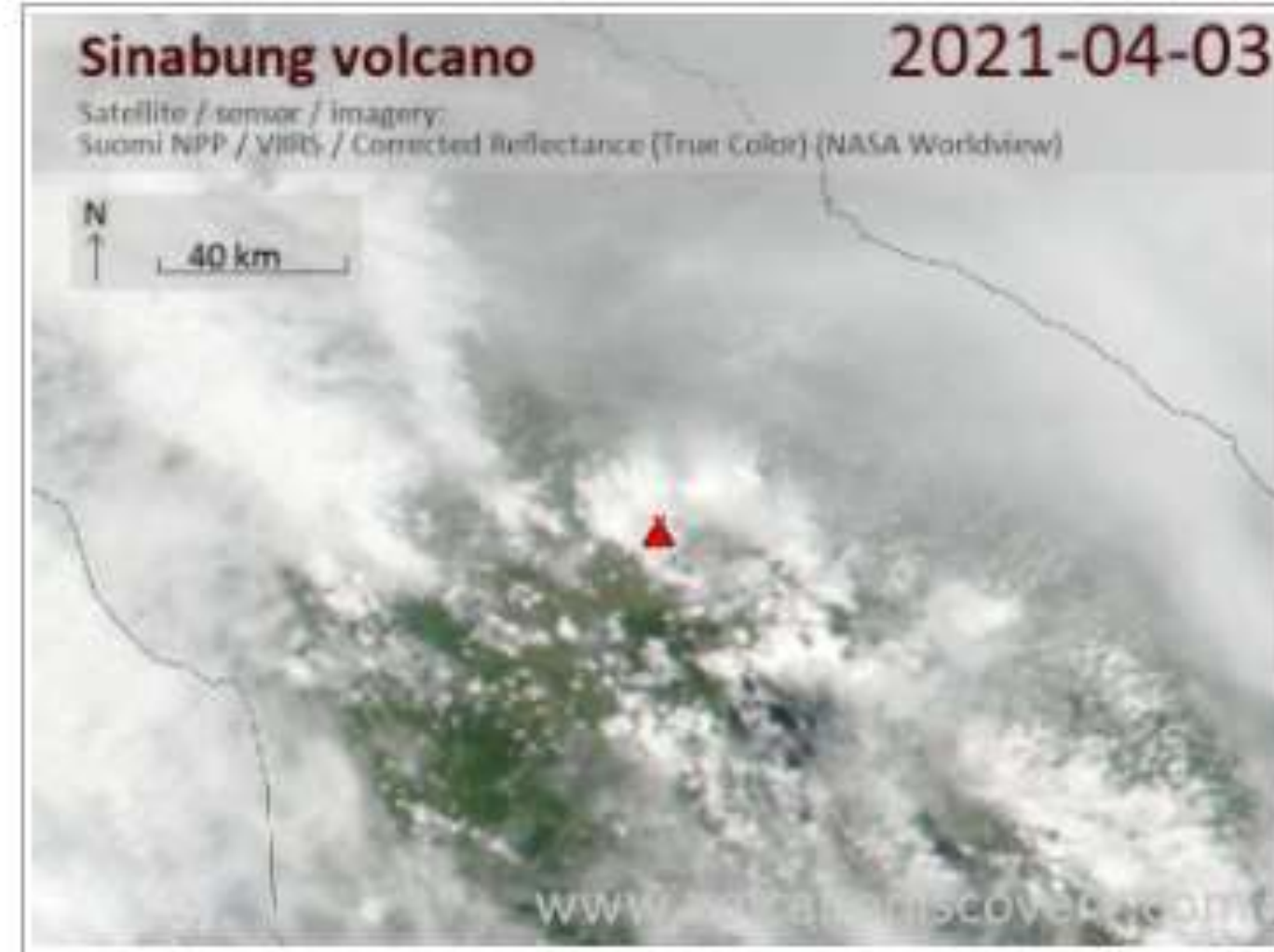
Satellite image of Sinabung volcano on 4 Apr 2021
