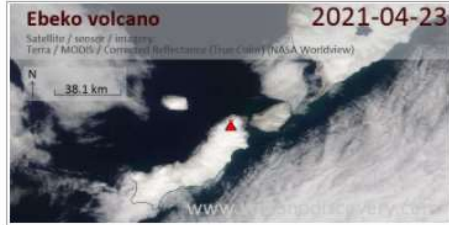
Satellite image of Ebeko volcano on 23 Apr 2021
