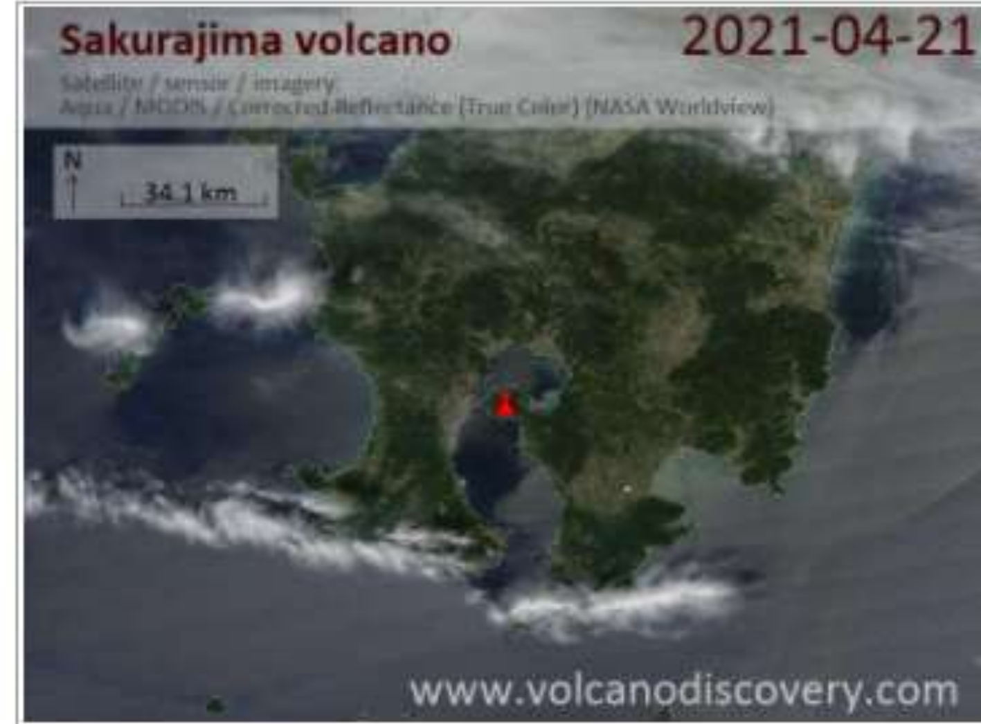
Satellite image of Sakurajima volcano on 22 Apr 2021
