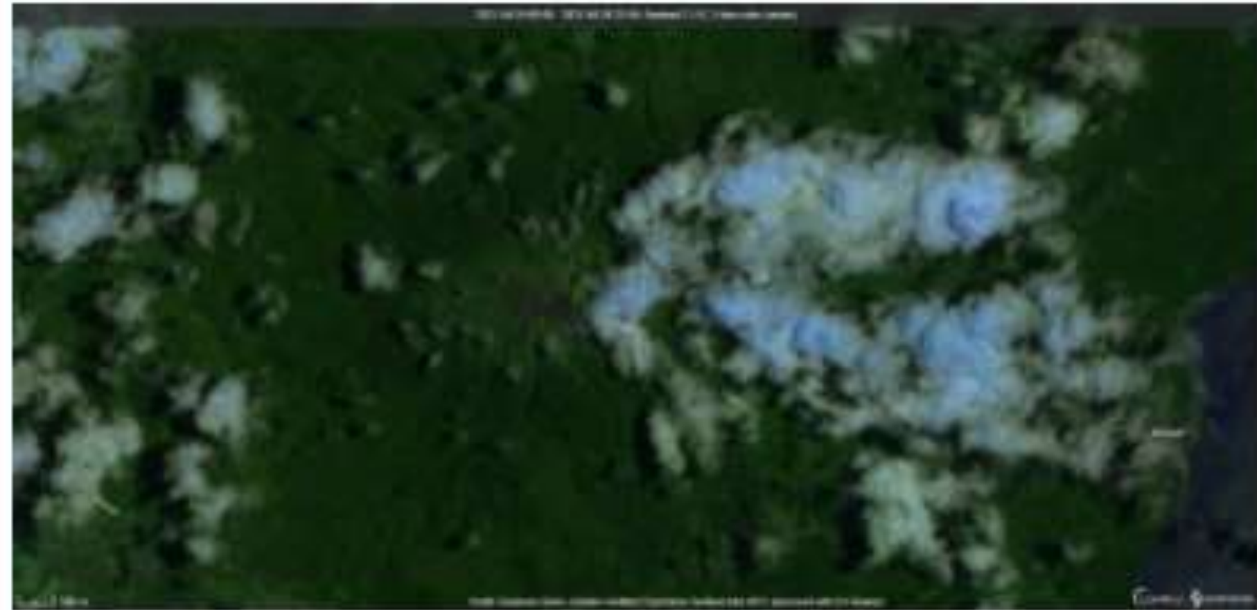
Satellite view of Bulusan volcano (image: Sentinel 2)
