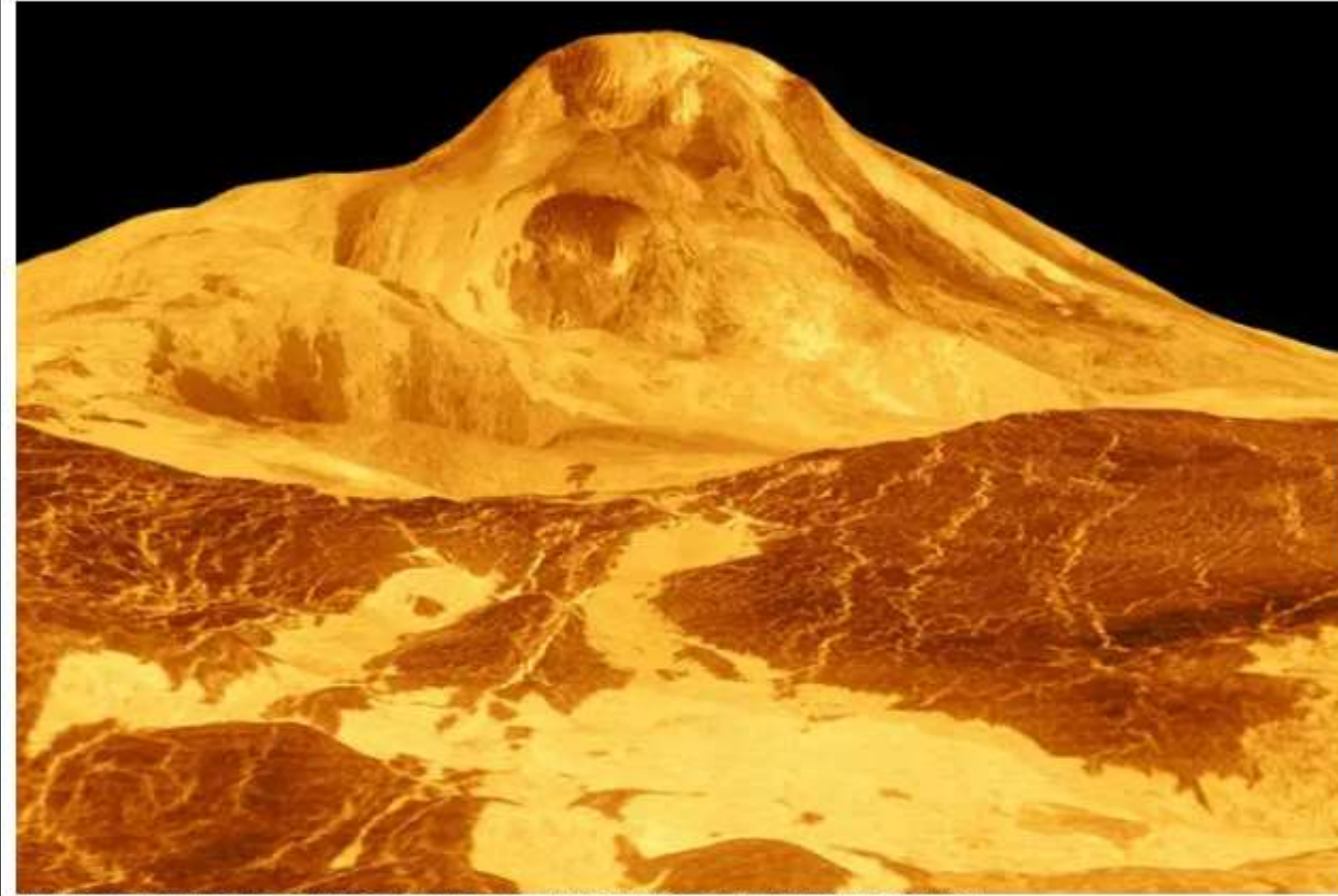
Maat Mons, a large volcano on Venus, in a simulated-color radar image from NASA's Magellan spacecraft. NASA/JPL
