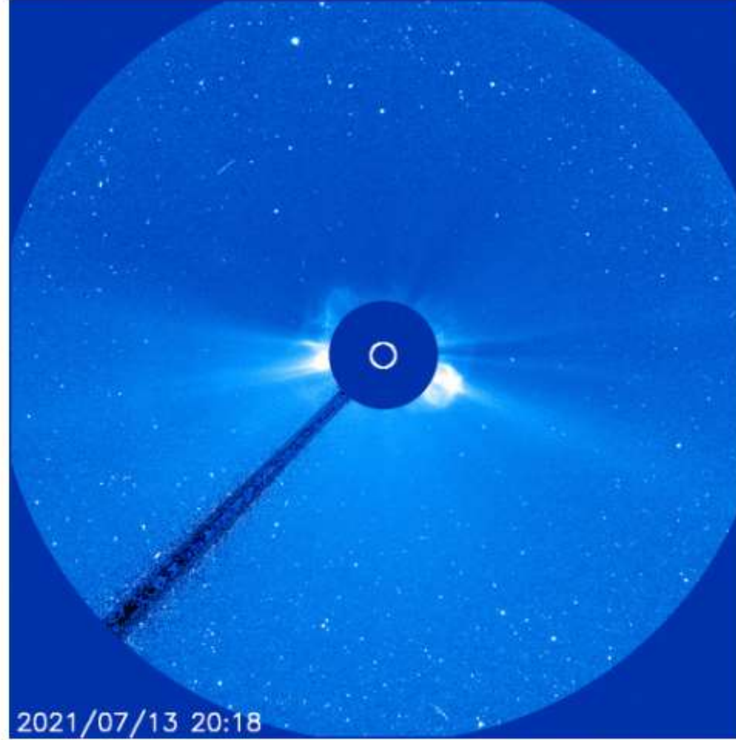
Above: The July 13th CME imaged by SOHO coronagraphs
