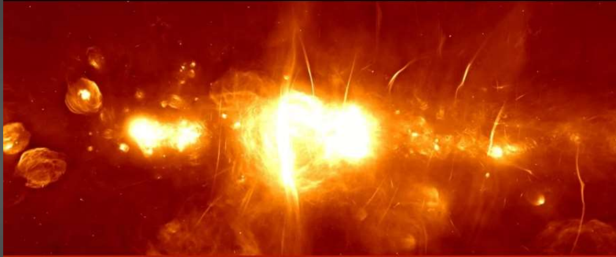
The galactic center in radio wavelengths. (MeerKAT/SARAC)
