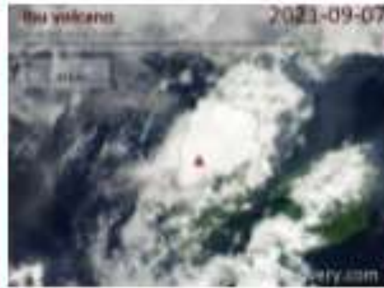
Satellite image of Ibu volcano on 7 Sep 2021
