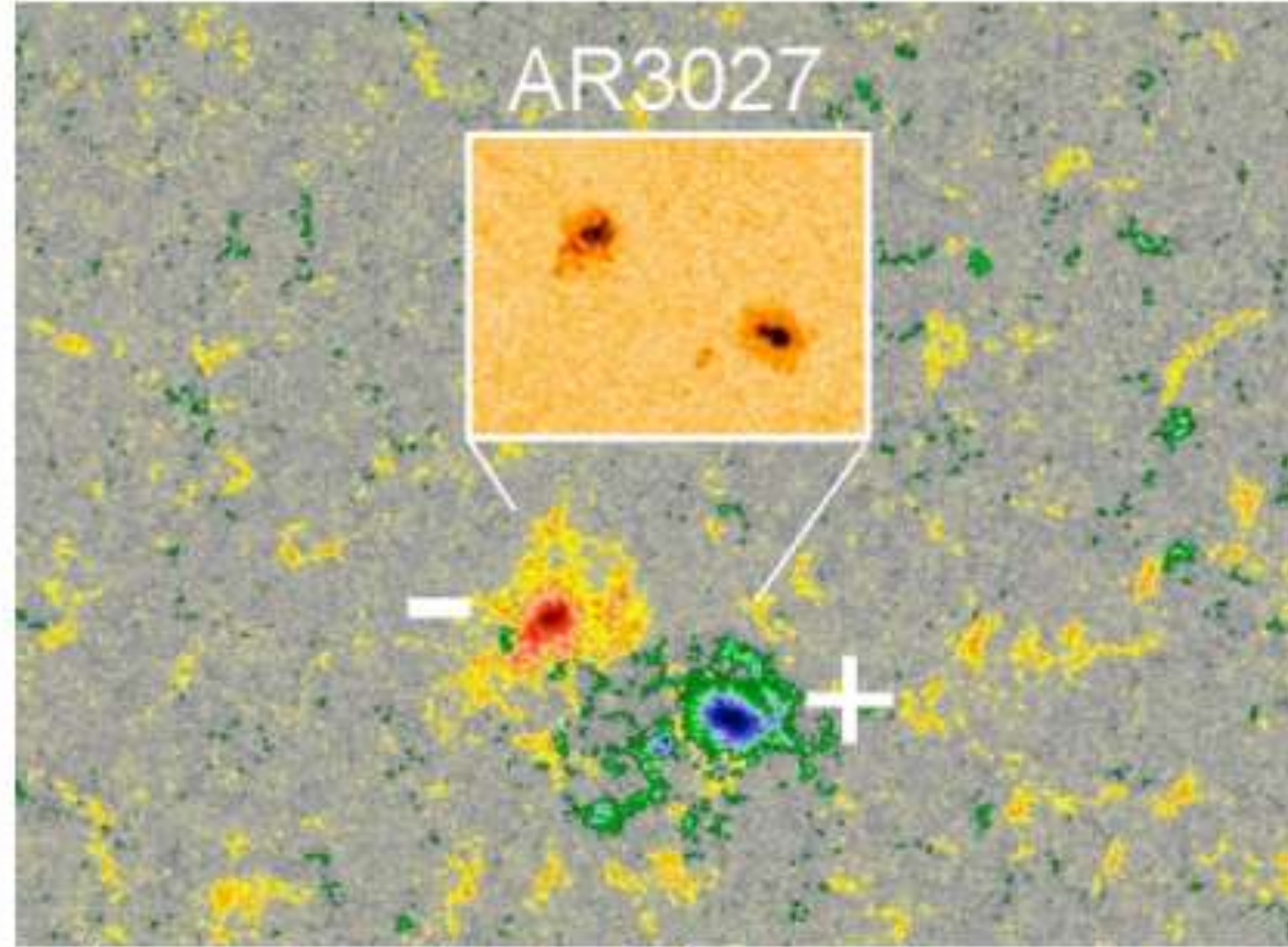
Above: A magnetic map of the sun's surface from NASA's Solar Dynamics Observatory.
