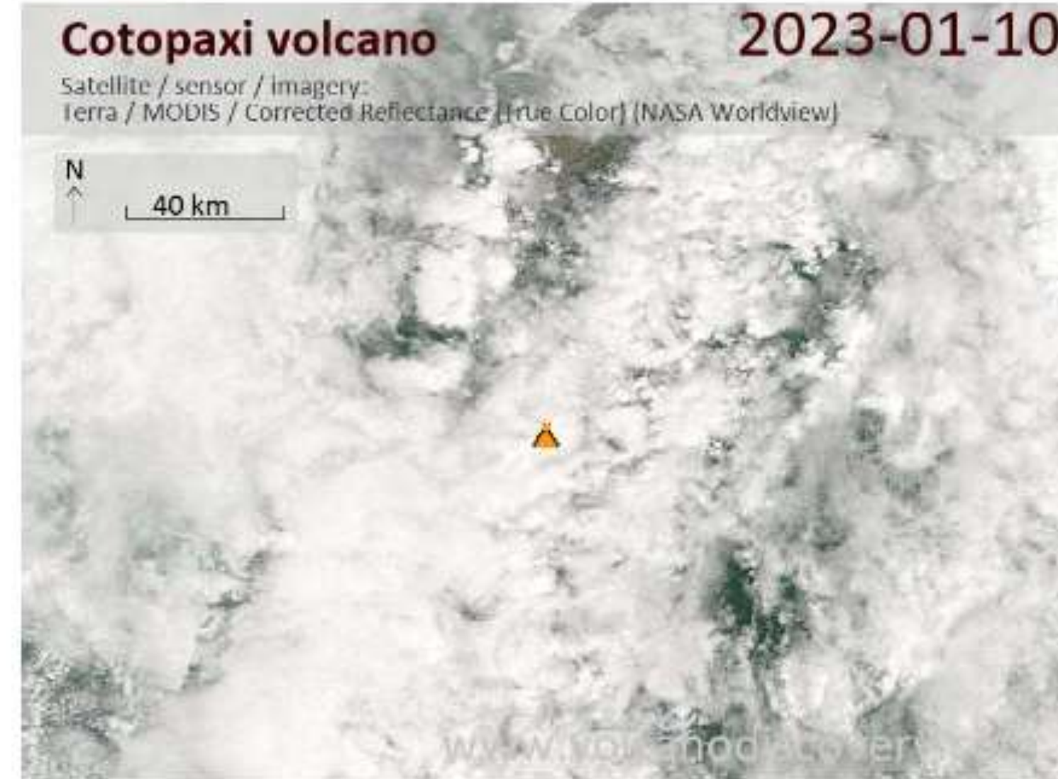
Satellite image of Cotopaxi volcano on 10 Jan 2023
