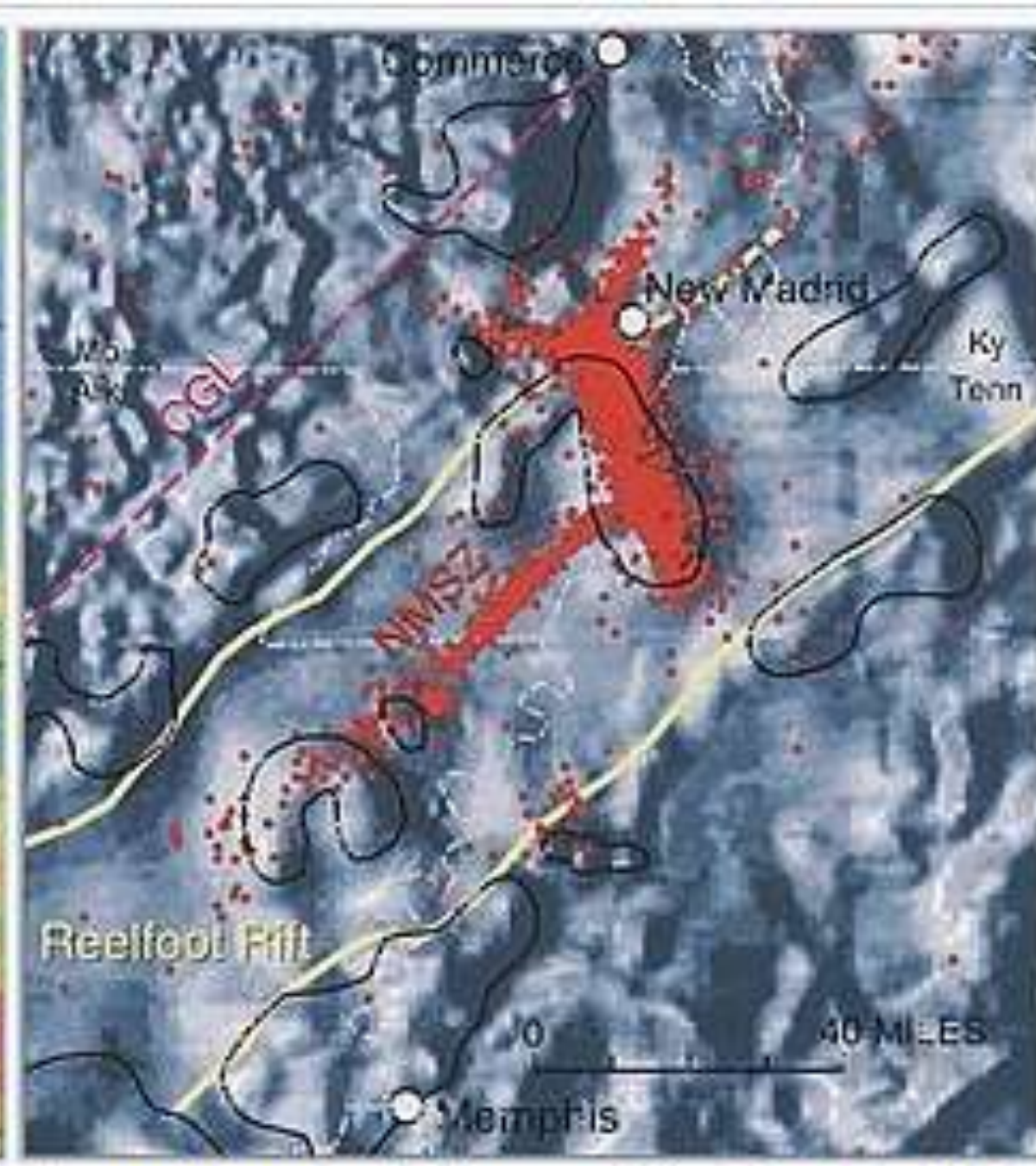
Magnetic potential map of the Reelfoot Rift
