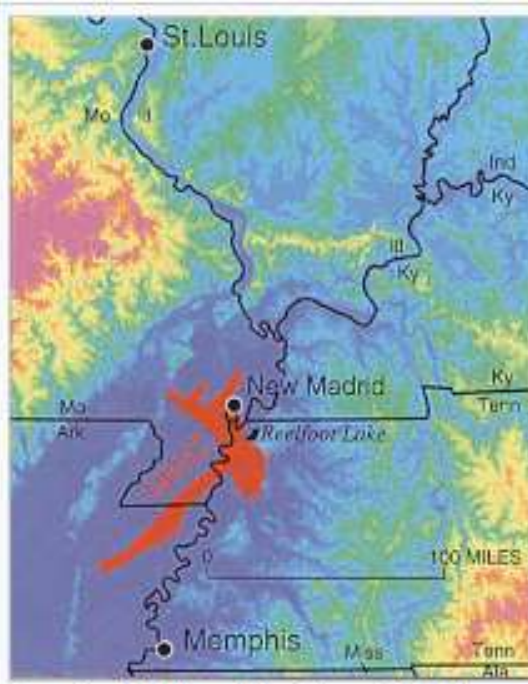
Reelfoot Rift and the New Madrid Seismic Zone in a 3D topographic image
