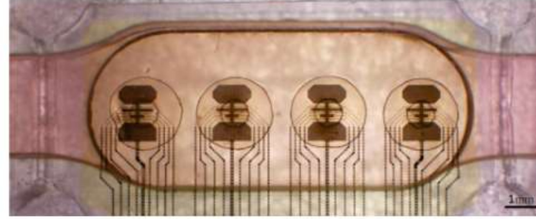
The bioprocessor with eight electrodes attached to four arrays each housing a cluster of brain cells. (Jordan et al., Frontiers in Artificial Intelligence, 2024)
