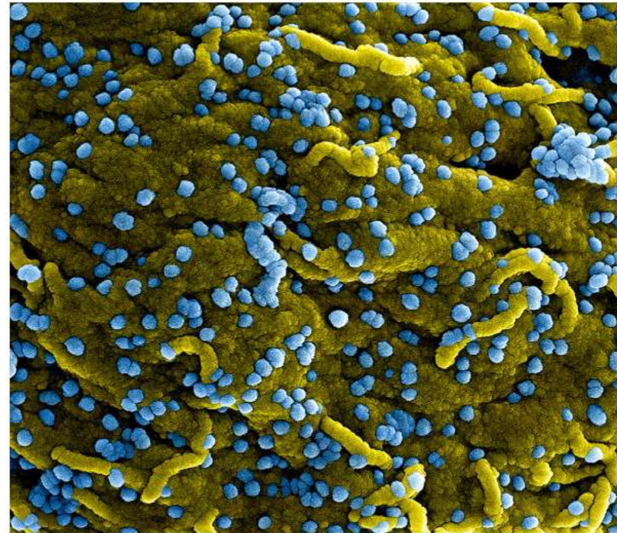
A colorized scanning of an electron micrograph shows Marburg virus particles (in blue) both budding and attached to the surface of infected cells (in yellow). Image
