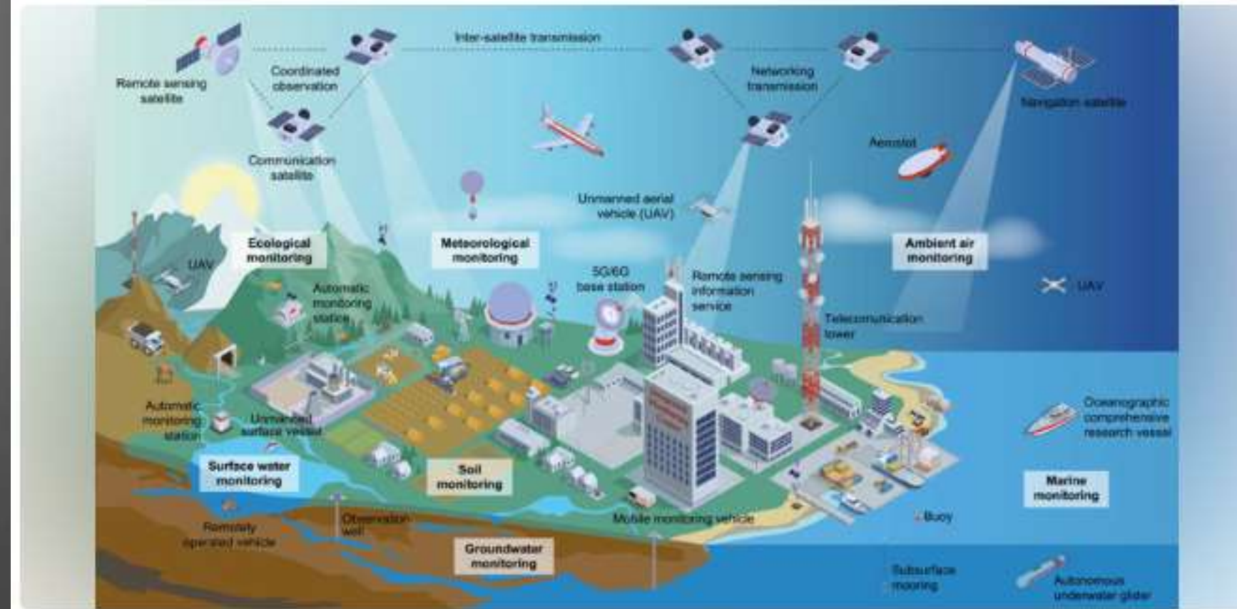
Schematic diagram of the Space-Air-Ground-Sea integrated eco-environment monitoring network. Credit: Environmental Science and Ecotechnology (2025). DOI: 10.1016/j.jese.2025.100585
