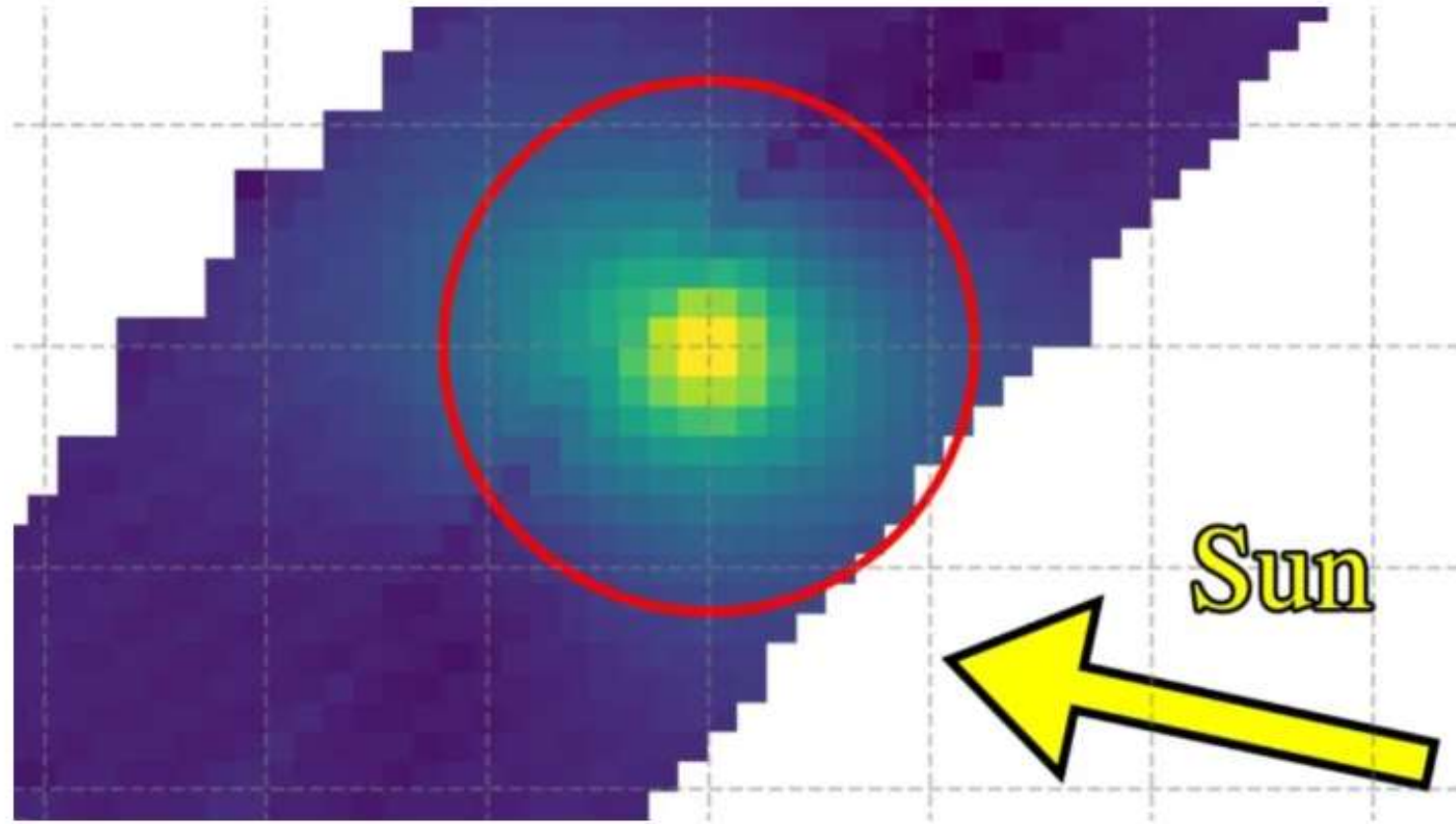
Image of 3I/ATLAS taken by the Keck Cosmic Web Imager (KCWI) on the Keck II telescope in Hawaii at the wavelength range of 0.3425 to 0.55 micrometers on August 24, 2025. The yellow arrow points in the direction of the Sun. Credit: W. B. Hoogendam et al. 2025
